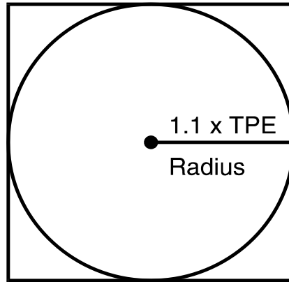
Figure H-24 Manual Solution for Square Search Area - Based on an Optimal Search Factor of 1.1
