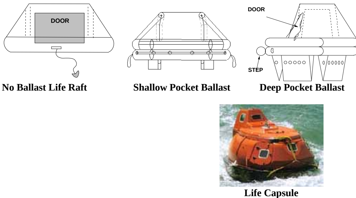
Figure H-2 Maritime Survival Craft
