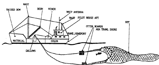
Side Trawler
