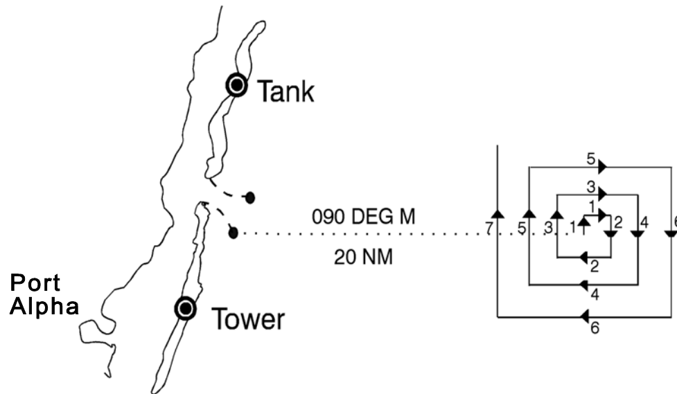
Figure H-43 Square Pattern Single-Unit (SS)
