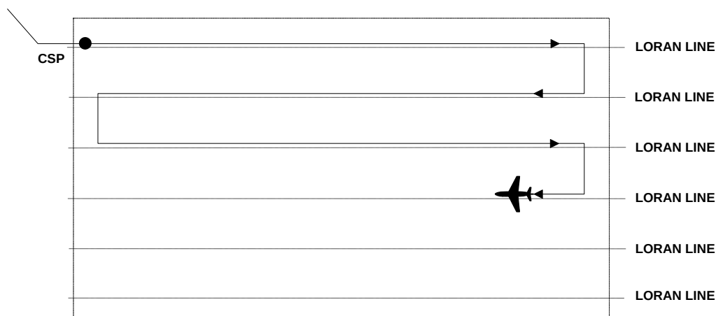
Figure H-38 Parallel Track Single-Unit LORAN (PSL)
