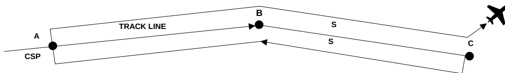
Figure H-30 Trackline Single-Unit Non-Return (TSN)
