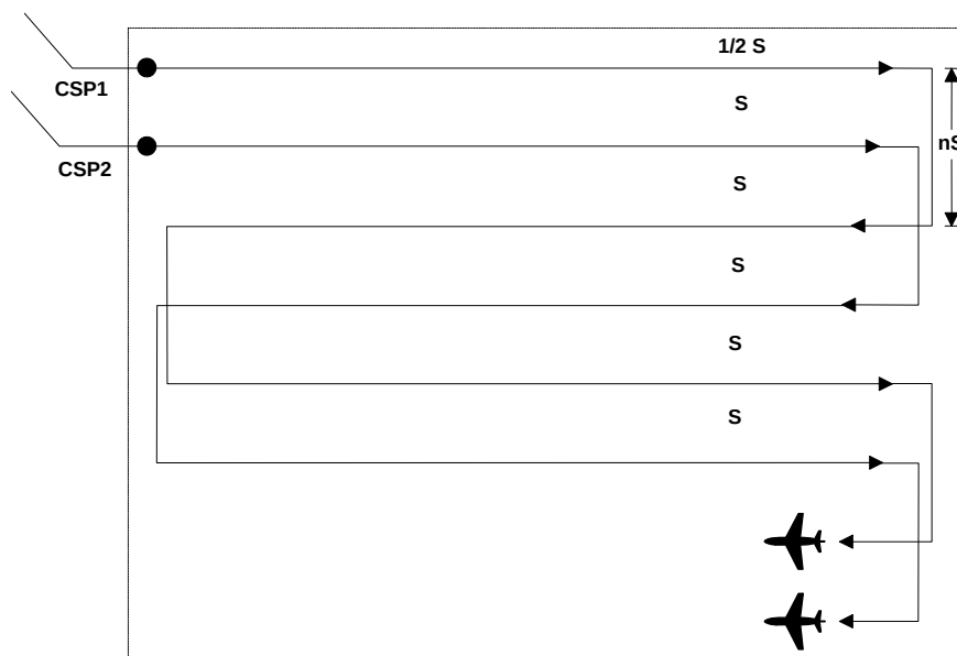
Figure H-35 Parallel Track Multi-Unit (PM)
